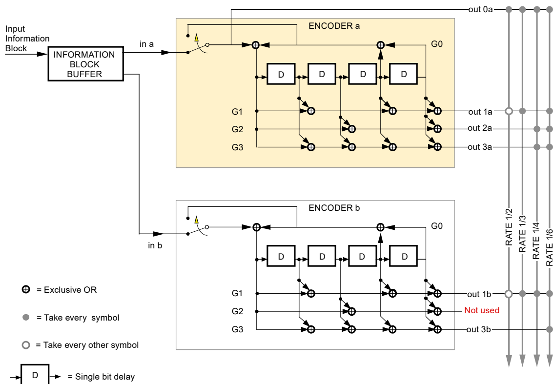
Figure 7-2: Turbo Encoder Block Diagram
