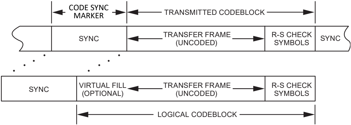
Figure 5-1: Reed-Solomon Codeblock Partitioning
