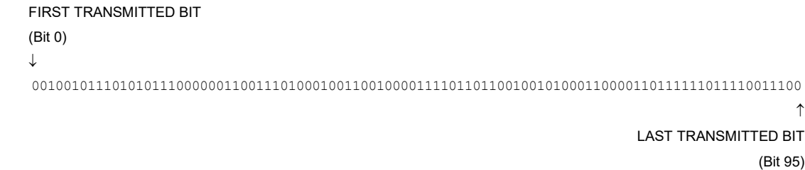
Figure 9-3: CSM Bit Pattern for Rate 1/3 Turbo Coded Data
