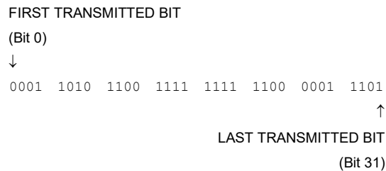
Figure 3-2: ASM Bit Pattern When Slicing is Used
