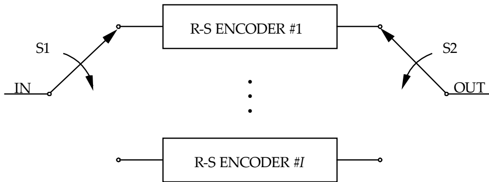
Figure 5-2: Functional Representation of R-S Interleaving
