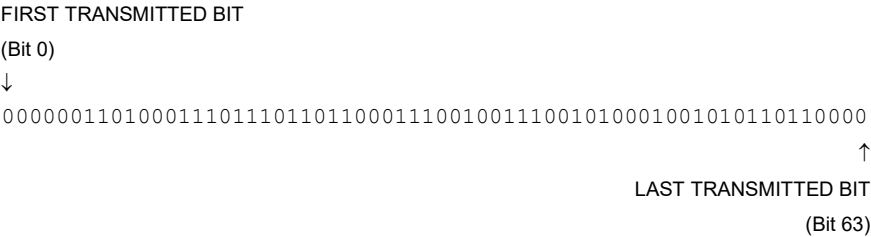
Figure 9-2: CSM Bit Pattern for Rate 1/2 Turbo and Rates 1/2, 2/3, and 4/5 LDPC Coded Data
