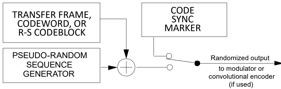
Figure 10-1: Pseudo-Randomizer Configuration
