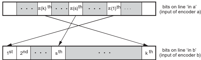
Figure 7-1: Interpretation of Permutation
