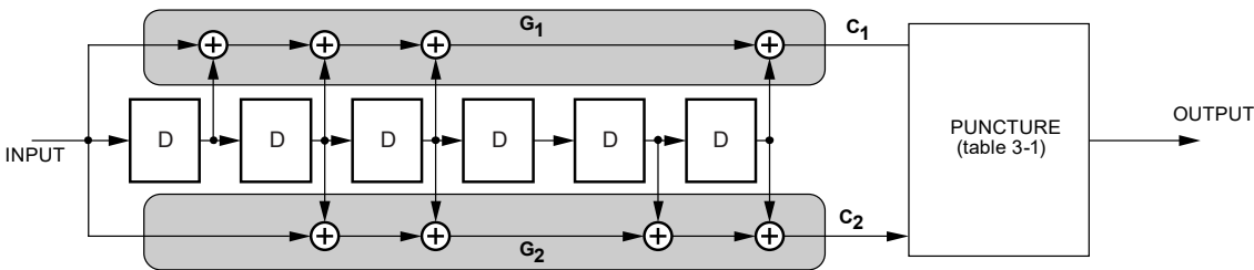
Figure 4-2: Punctured Encoder Block Diagram
