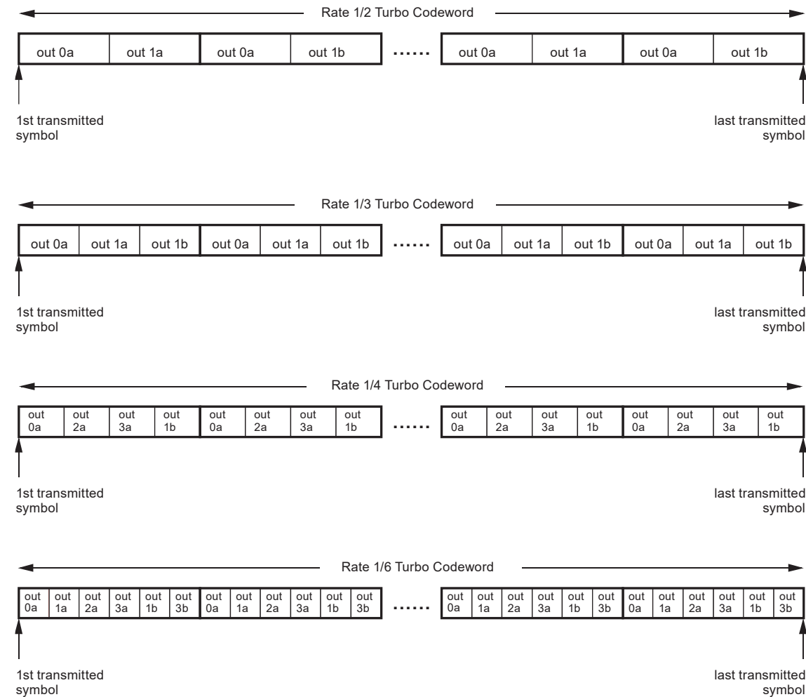
Figure 7-3: Turbo Codewords for Different Code Rates
