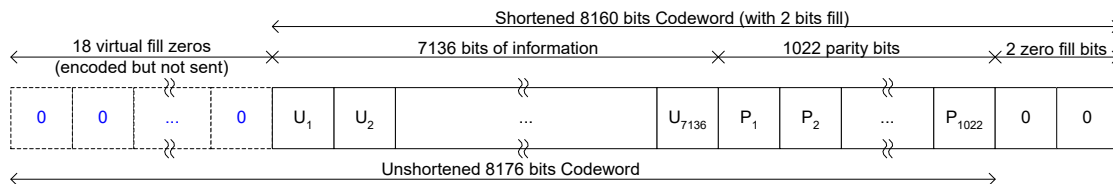
Figure 8-3: Shortened Codeword
