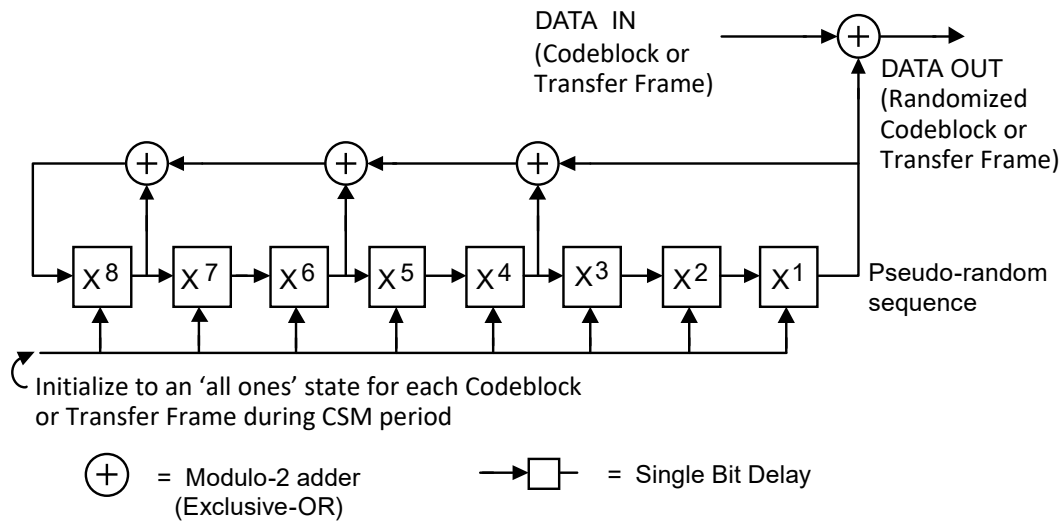
Figure 10-3: Pseudo-Randomizer Logic Diagram for the 255-Bit Sequence (Only for Backward Compatibility with Legacy Systems)
