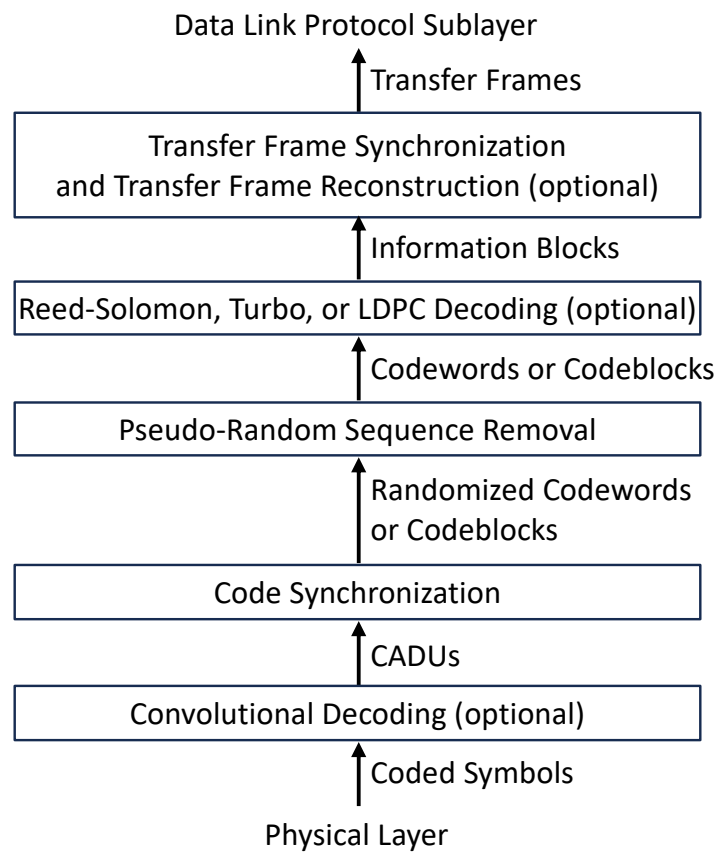
Figure 2-4: Internal Organization of the Sublayer at the Receiving End
