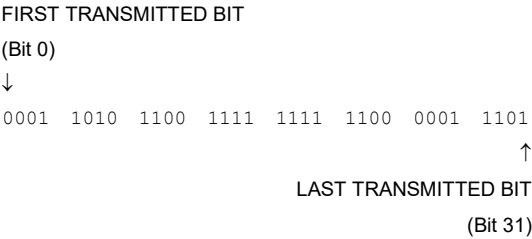
Figure 9-1: CSM Bit Pattern for Uncoded, Convolutional, Reed-Solomon, Concatenated, and Rate 7/8 LDPC Coded Data
